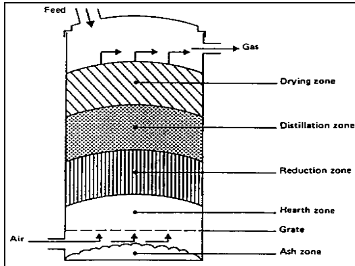
Figure II.2 Updraft Gasifier
