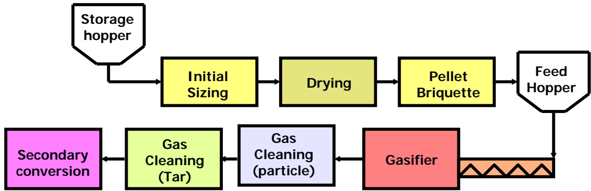
Figure I.1 Gasification Process [2]
