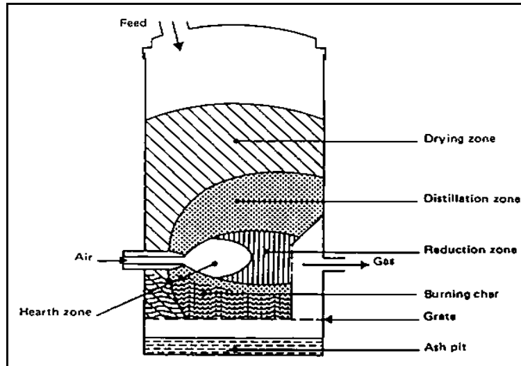
Figure II.4 Crossdraft Gasifier
